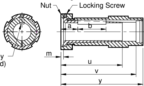
Thin Walled Bushing
