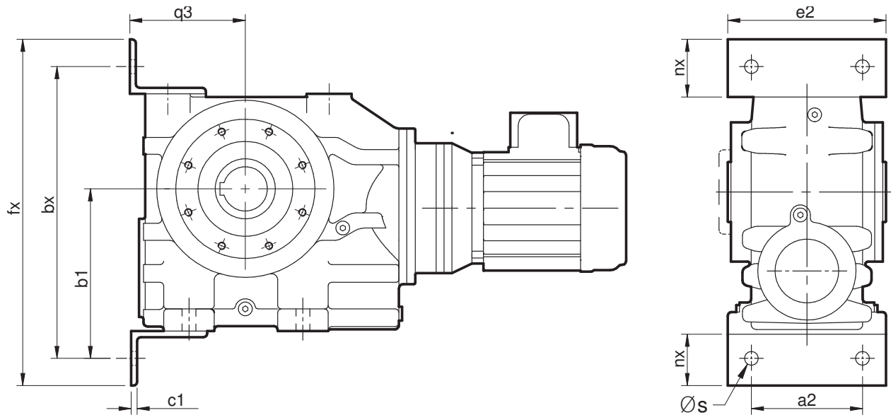
STANDARD UNIT WITH END MOUNTED FEET
