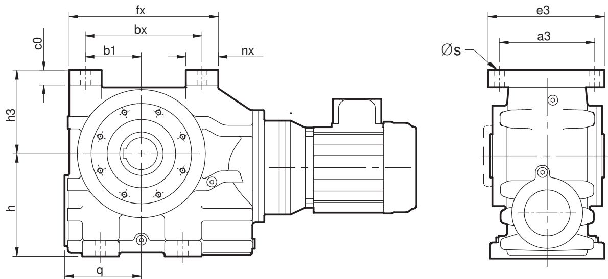
STANDARD UNIT WITH TOP MOUNTED FEET
