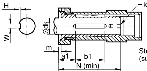
Driven Shaft
