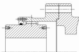
SHAPE OF COUPLING FOR SIZE 29000 & 56000
