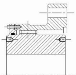
SHAPE OF GEAR HALF FOR COUPLING SIZE 29000
